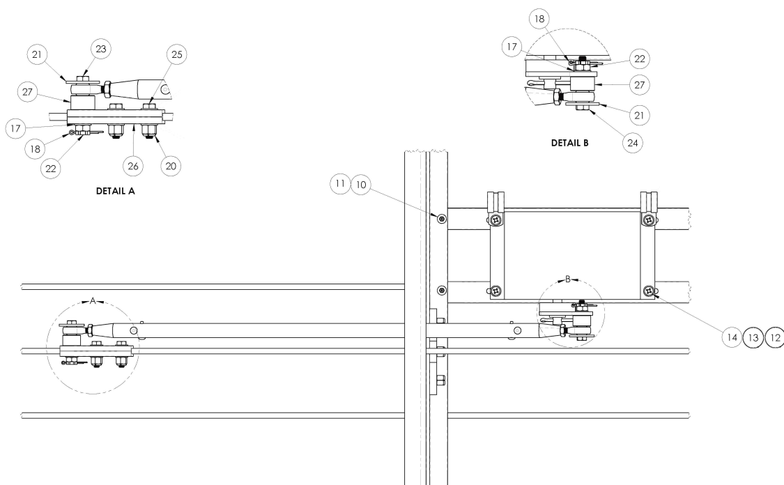
FIGURE 8 - OPTION 2 PITCH SERVO PROVISIONS
