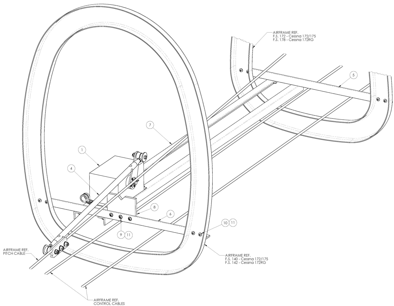
FIGURE 6 - OPTION 2 PITCH SERVO INSTALLATION
