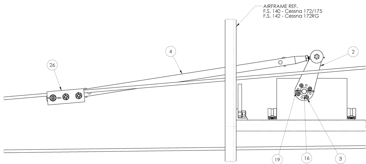
FIGURE 7 - OPTION 2 PITCH SERVO PROVISIONS
