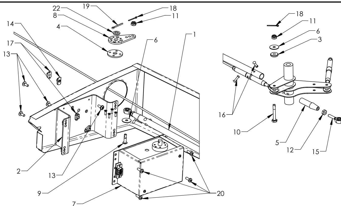
FIGURE 4 - ROLL SERVO PROVISIONS
