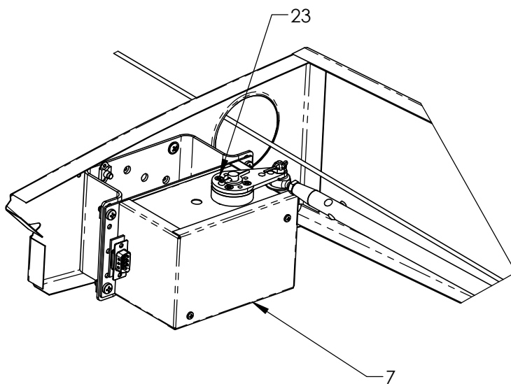
FIGURE 2 - ROLL SERVO INSTL
