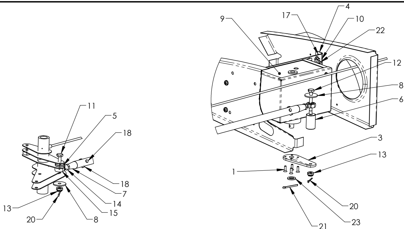
FIGURE 4 - ROLL SERVO INSTL
