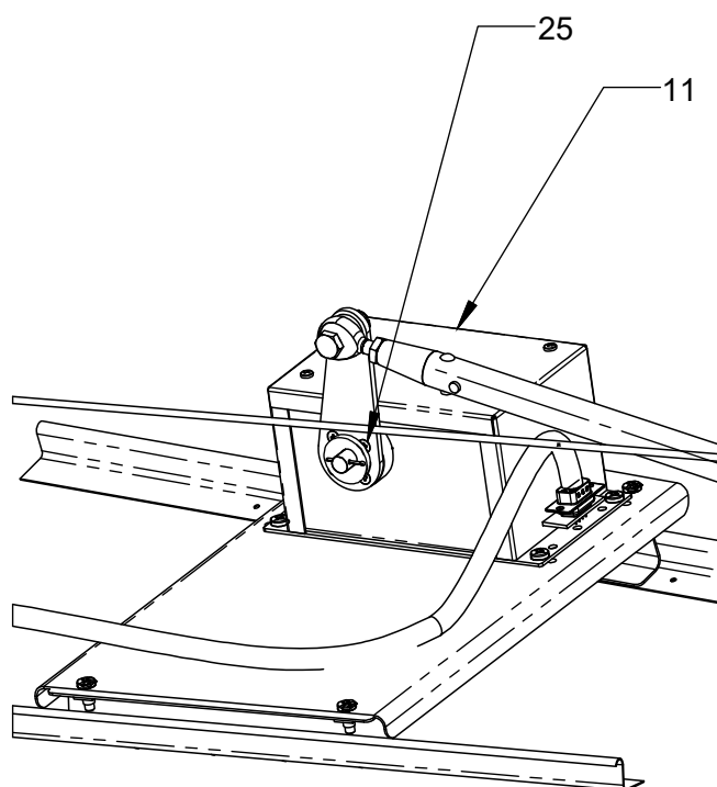
FIGURE 2 - ROLL SERVO INSTL
