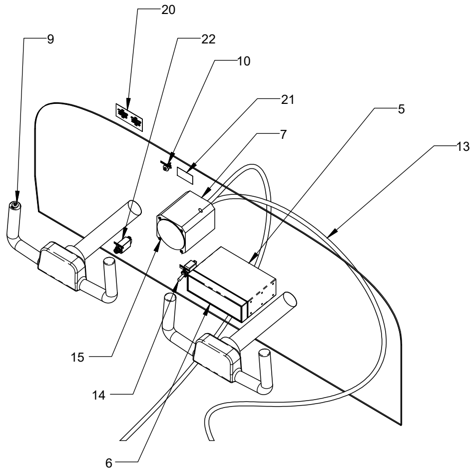
FIGURE 1 - INSTRUMENT PANEL
