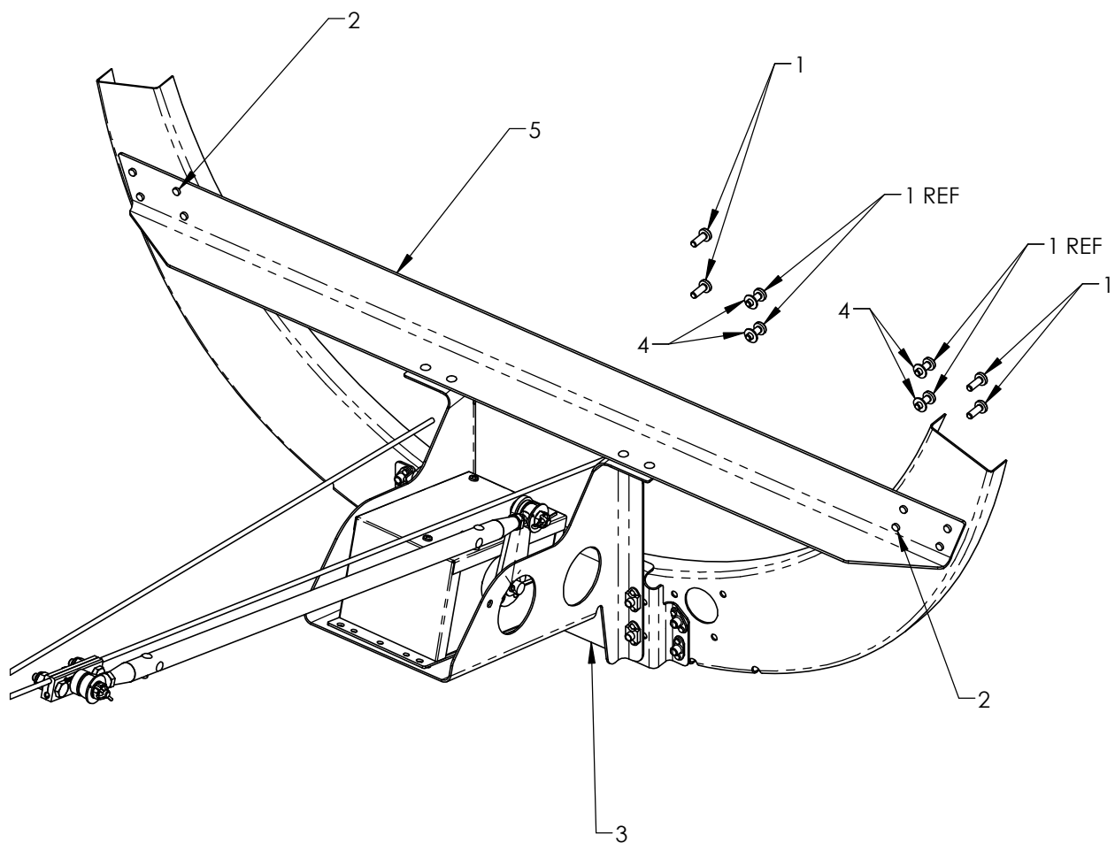
FIGURE 4 - PITCH SERVO MOUNTING (APPLICABLE TO MODELS 150 THRU 150C (AIRCRAFT SERIALS 17001 THRU 15060087))
