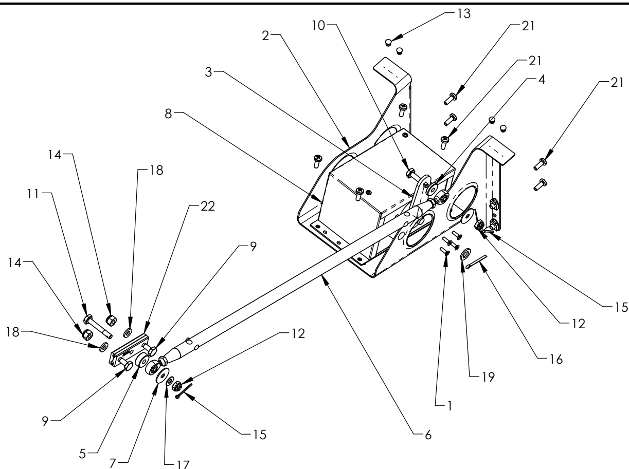
FIGURE 2 - PITCH SERVO INSTL
