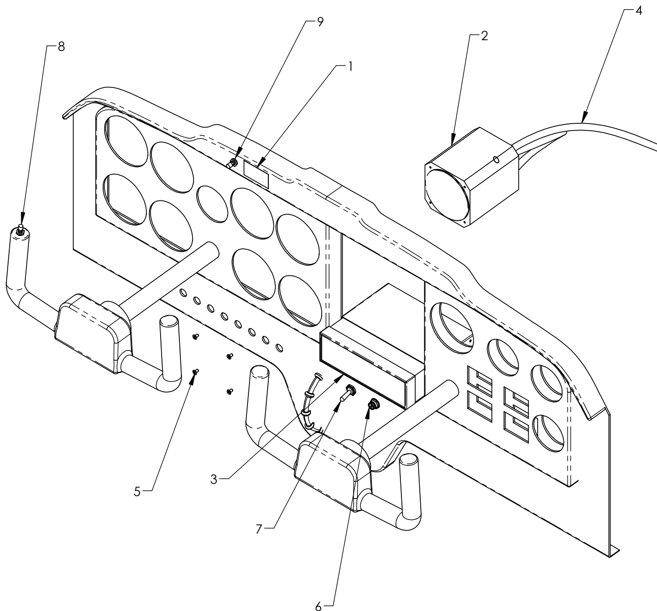
FIGURE 1 - INSTRUMENT PANEL
