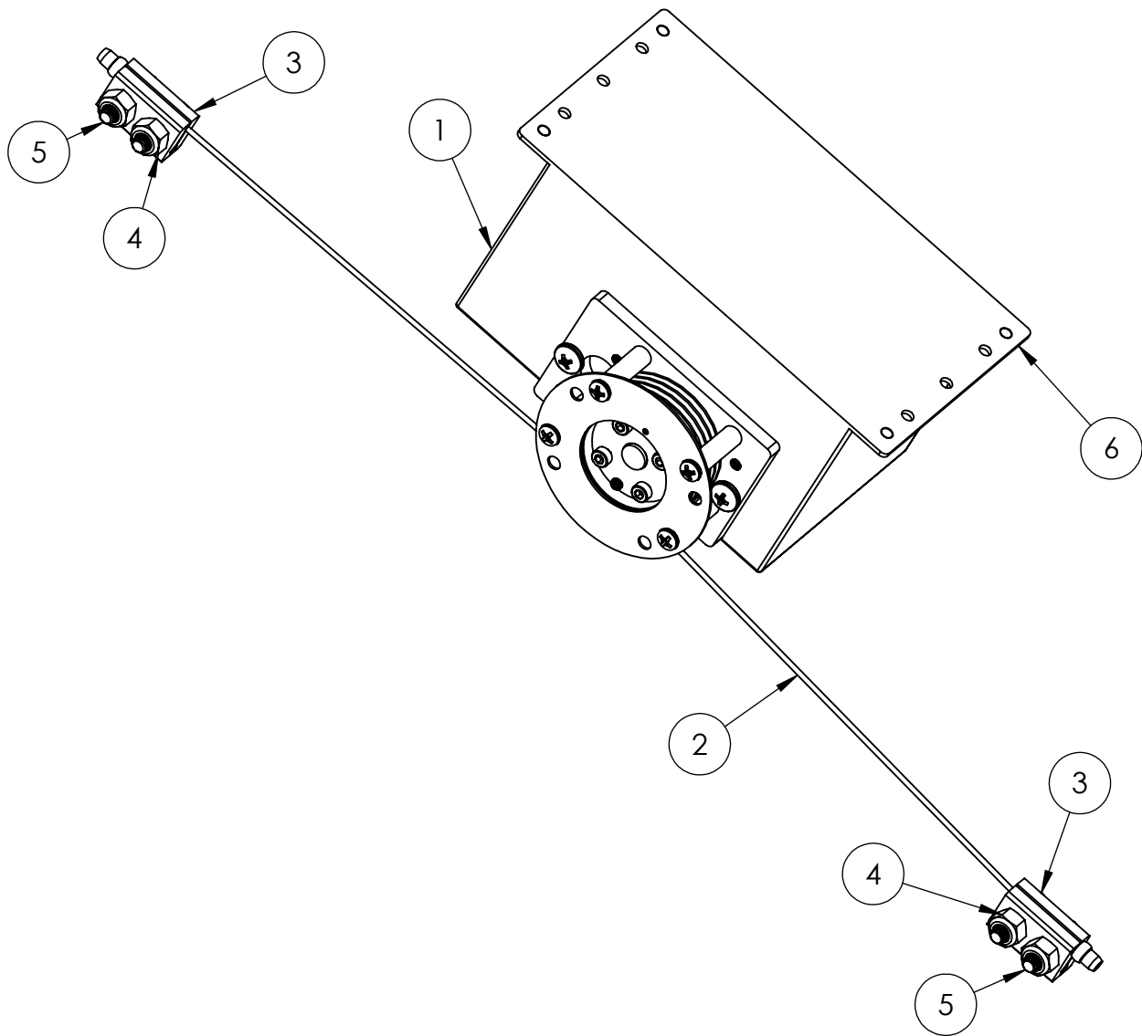
FIGURE #3 - ROLL SERVO ASSEMBLY DETAIL
