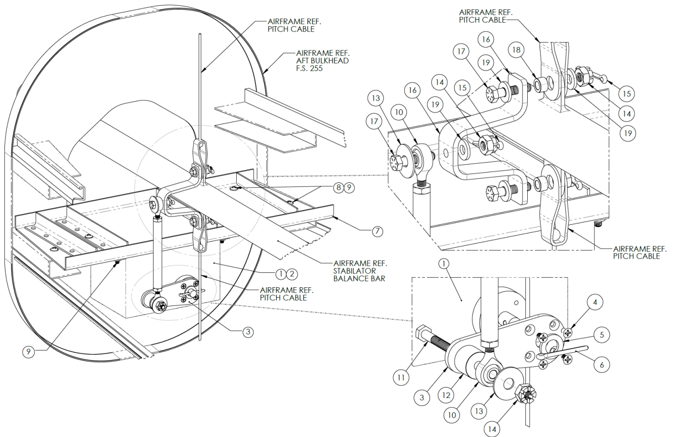
FIGURE 4 - PITCH SERVO PROVISIONS
