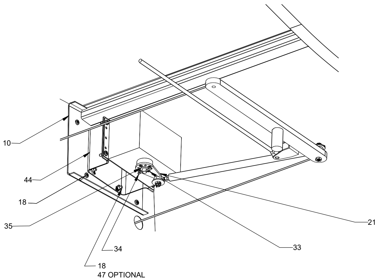
FIGURE 2 - ROLL SERVO INSTL
