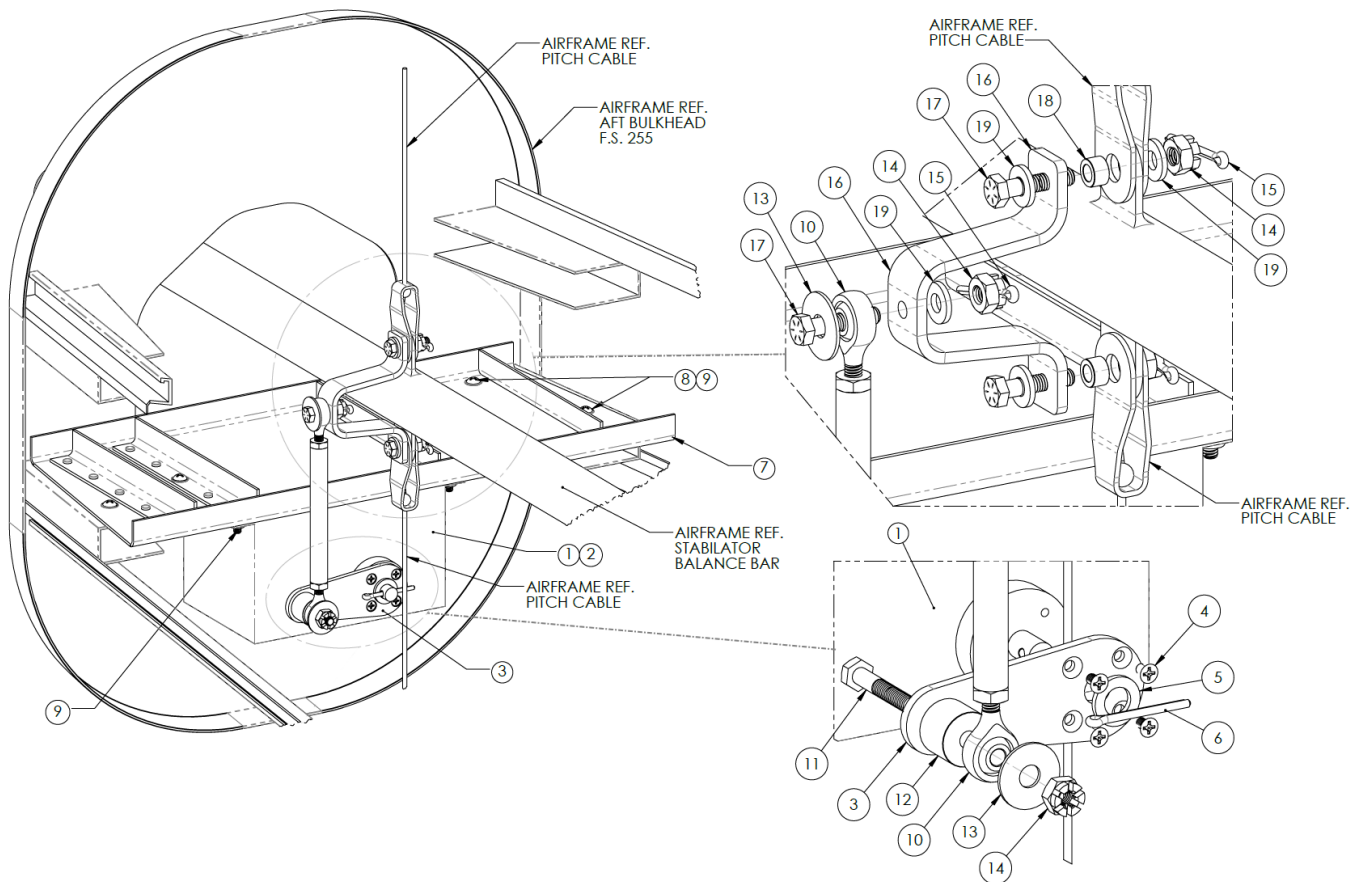
FIGURE 5 - PITCH SERVO PROVISIONS
