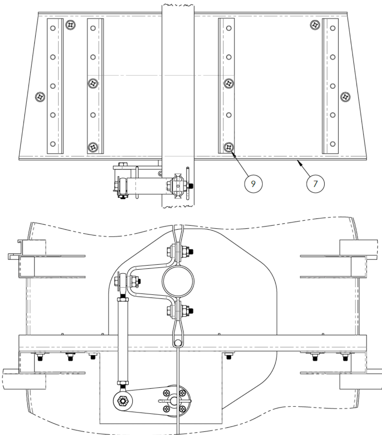
FIGURE 6 -PITCH SERVO INSTL
