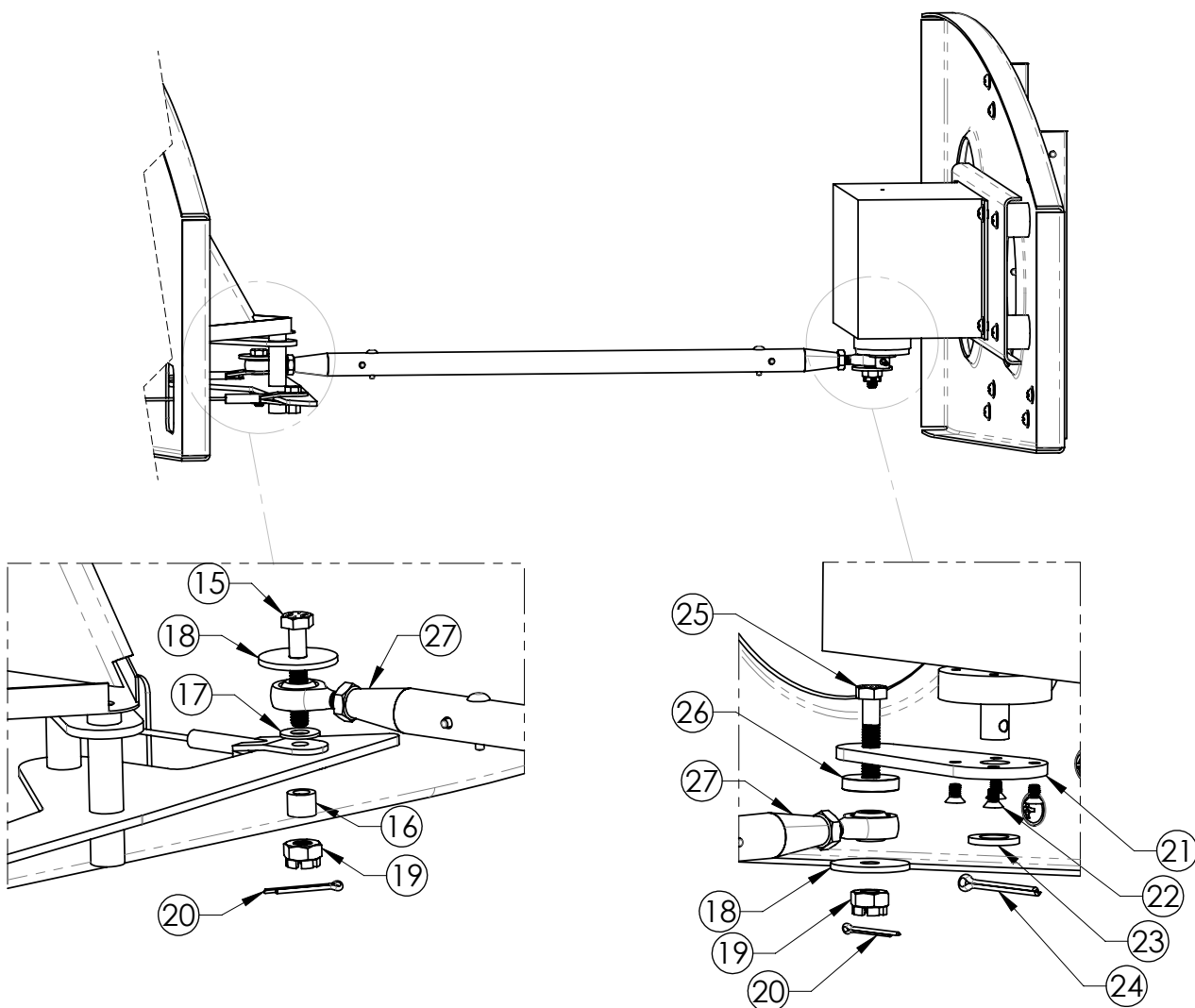
FIGURE 4 - ROLL SERVO PROVISIONS
