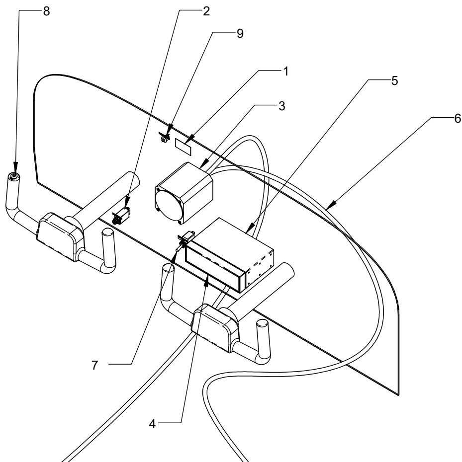
FIGURE 1 - INSTRUMENT PANEL
