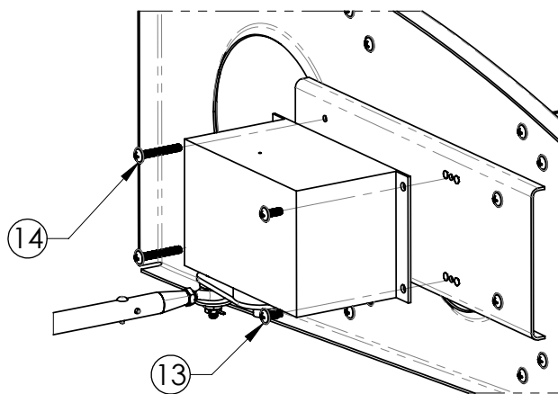
FIGURE 3 - ROLL SERVO PROVISIONS
