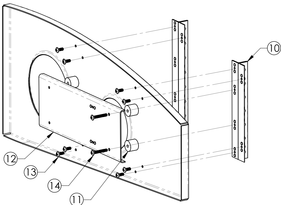
FIGURE 2 - ROLL SERVO PROVISIONS
