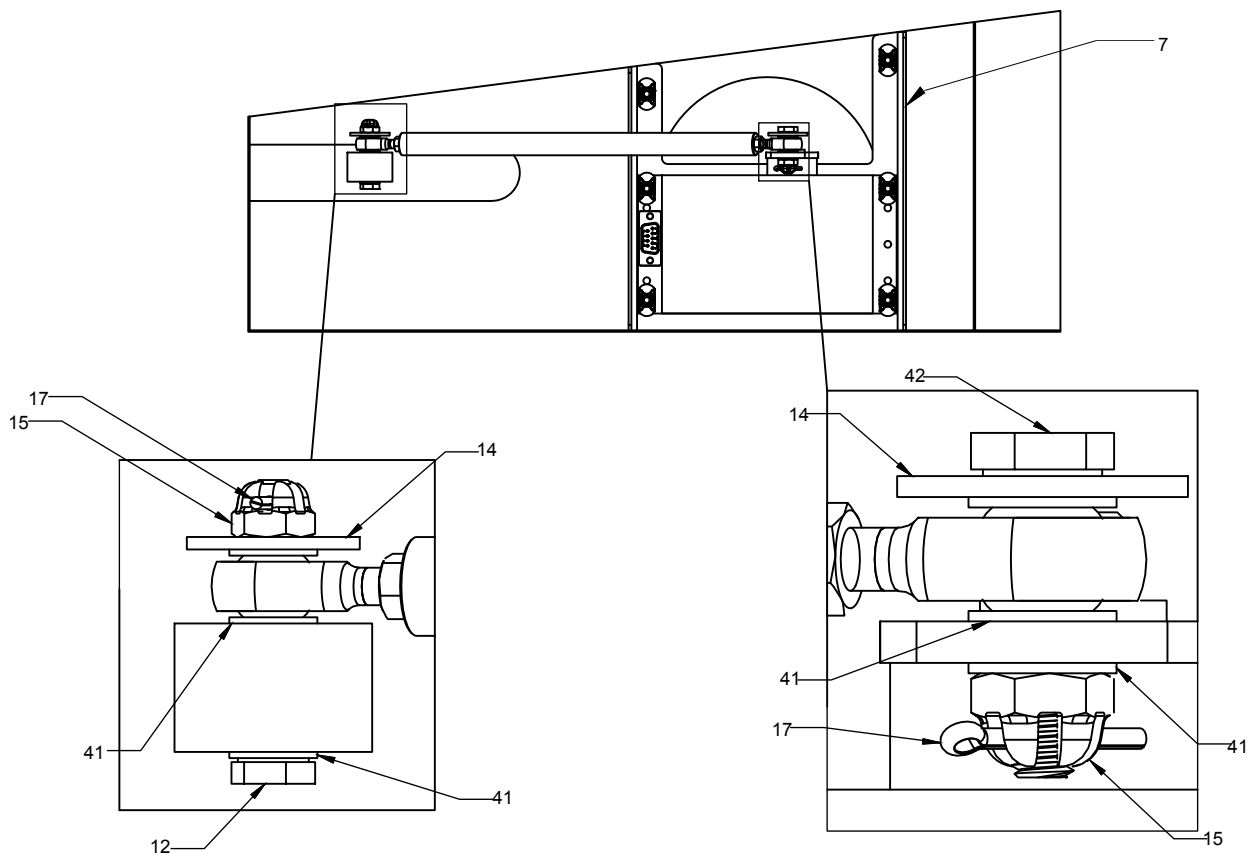
FIGURE 4 - ROLL SERVO PROVISIONS
