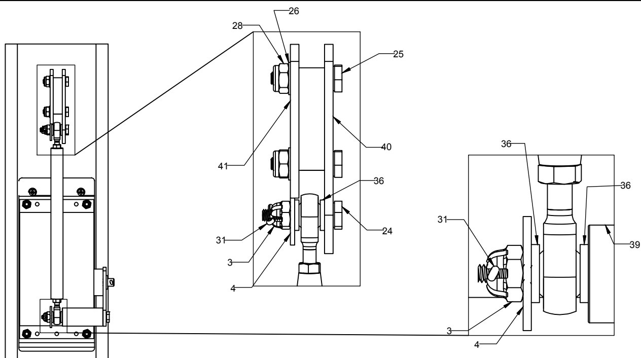
FIGURE 5 - PITCH SERVO PROVISIONS
