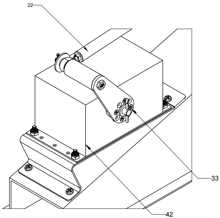
FIGURE 3 - PITCH SERVO INSTL
