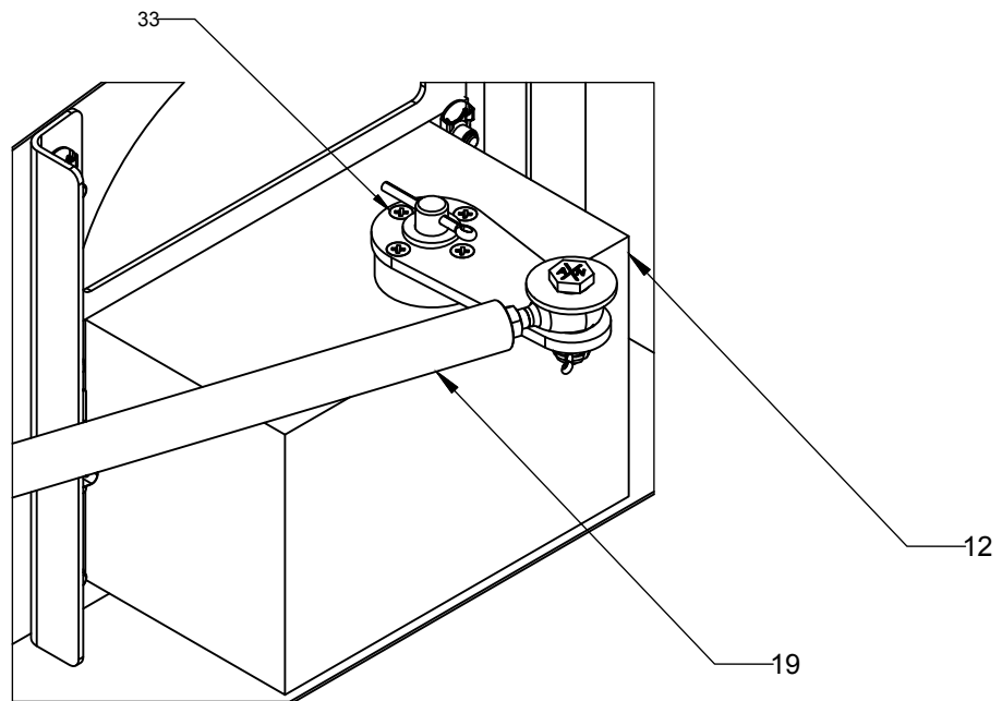
FIGURE 2 - ROLL SERVO INSTL
