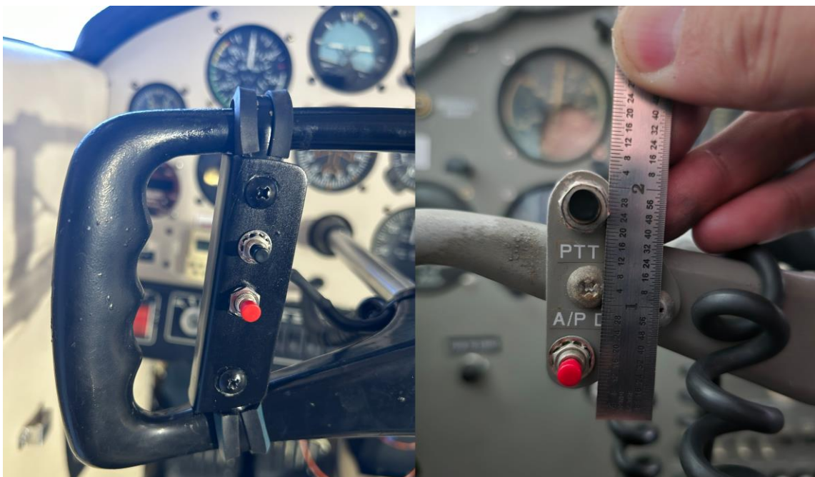
FIGURE 1 50'S & 60'S CESSNA 150/172/175
